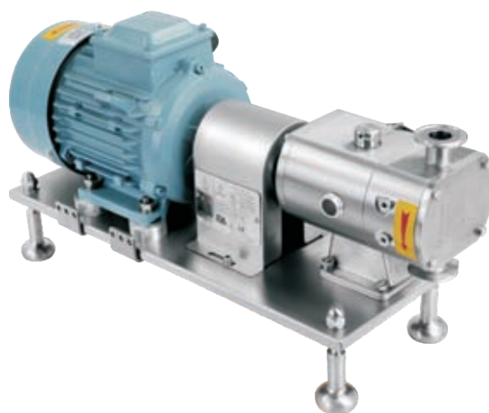
电机直连式-MINI转子泵 Motor direct connection type-MINI rotary lobe pump
