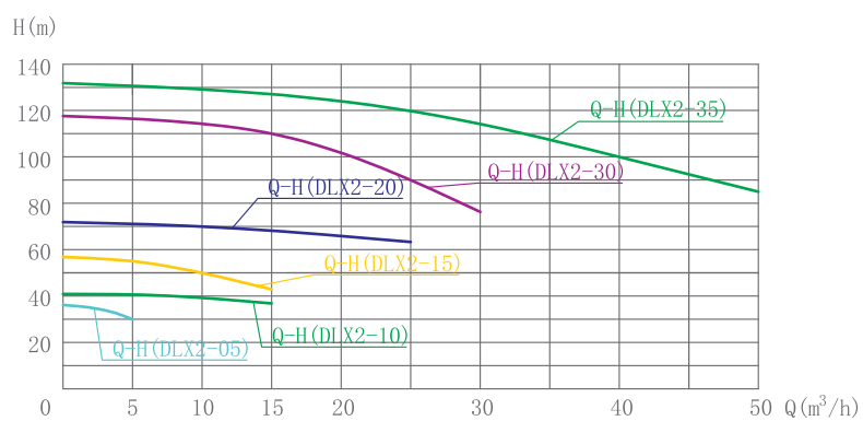
DJ-DLX-2系列离心泵Q-H曲线图 DJ-DLX-2 series centrifugal pump Q-H curve
