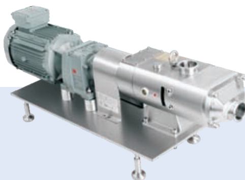
带电机减速机螺杆泵 Screw pump with motor and reducer
