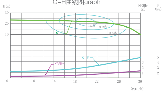
HLX-20(4P) Q-H曲线图graph
