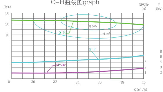
HLX-30(4P) Q-H曲线图graph
