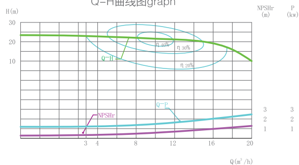
HLX-15(4P) Q-H曲线图graph
