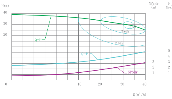
BS-12(Q-H曲线图graph)
