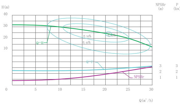
BS-6(Q-H曲线图graph)
