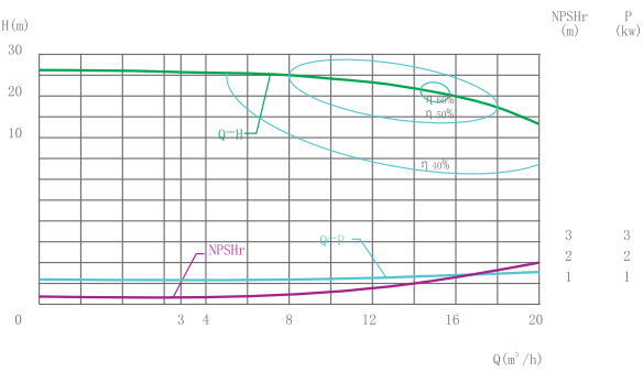
BS-4(Q-H曲线图graph)
